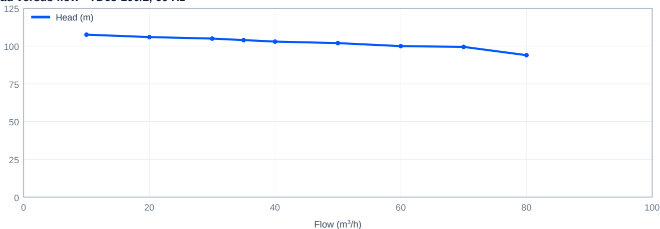
Head versus flow - TD65-100/2, 60 Hz
