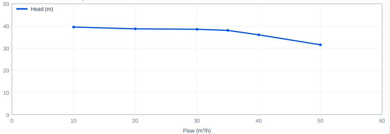
Head versus flow - TD65-38/2, 60 Hz
