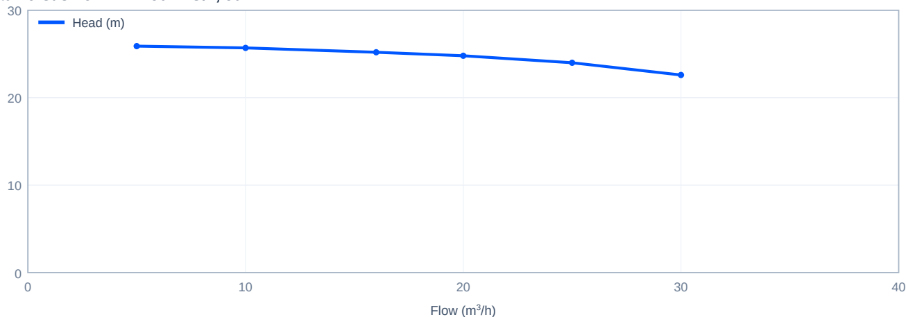
Head versus flow - TDE50-24G/2, 50 Hz
