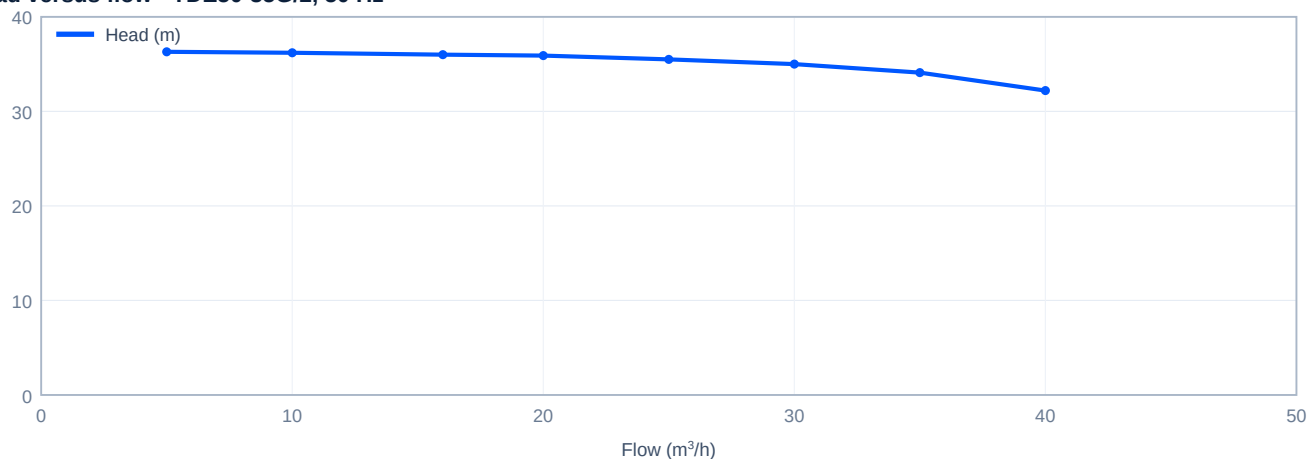
Head versus flow - TDE50-35G/2, 50 Hz
