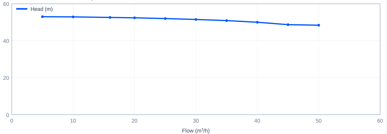
Head versus flow - TDE50-50G/2, 50 Hz
