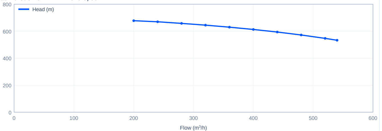
Head versus flow - VMHP520-5, 50 Hz
