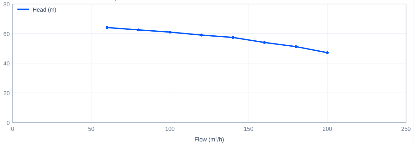
Head versus flow - ZS100-80-200/37.0, 50 Hz
