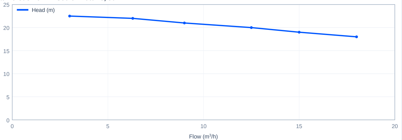
Head versus flow - ZS50-32-160/1.5, 50 Hz
