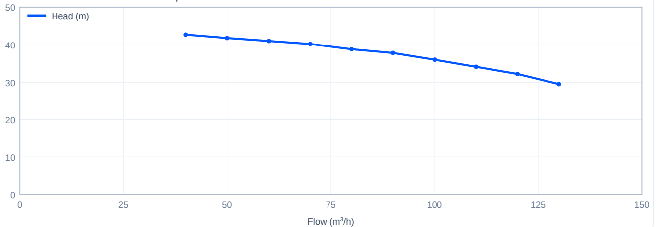
Head versus flow - ZS80-65-160/15.0, 60 Hz
